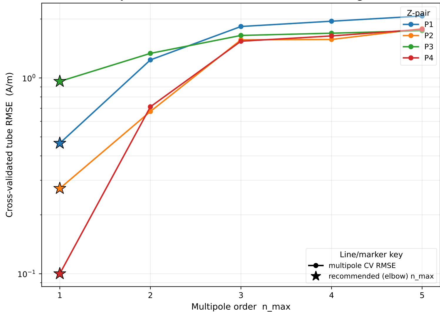
Multipole RMSE vs. Order — Cross-Pair Convergence
